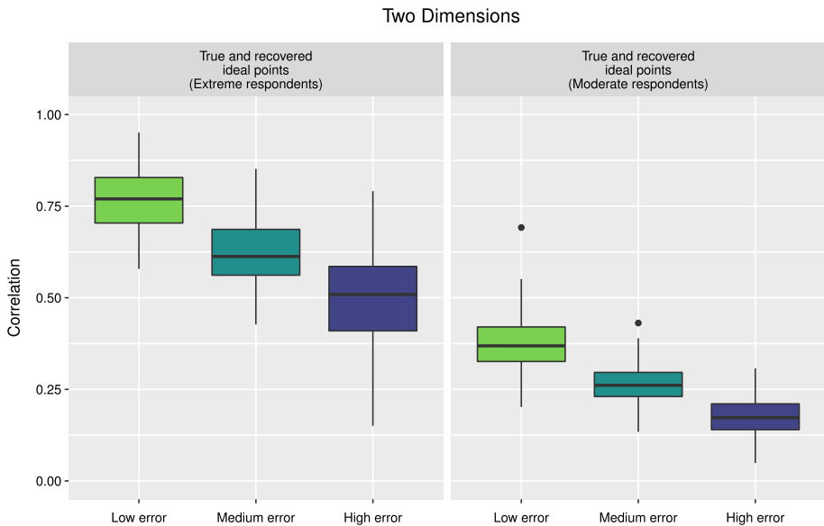
Fig. 7 Monte Carlo tests of Ordered Optimal Classification recovery of ideologically moderate and extreme respondents' ideal points
