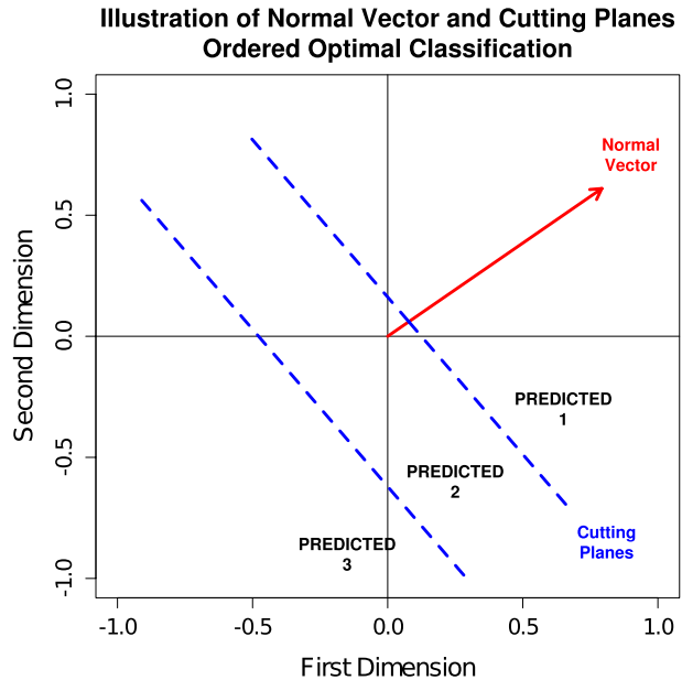
Fig. 2 Illustration of Ordered Optimal Classification. A single normal vector is estimated for each survey item, and the c - 1 cutting planes (where c is the number of response categories in the corresponding item) continue to be restricted to be perpendicular to the normal vector
