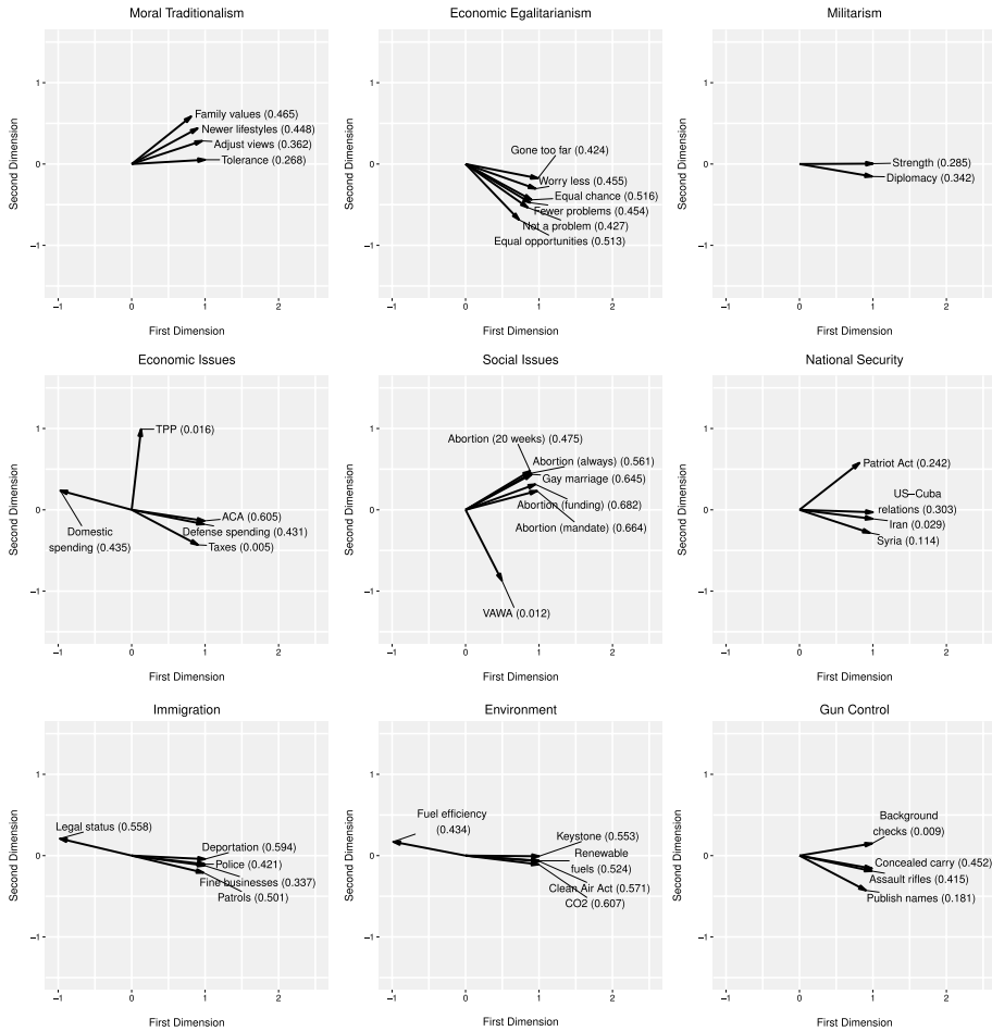
Fig. 6 Selected normal vectors from Ordered Optimal Classification scaling of the 2015 Cooperative Congressional Election Study. Arrows denote the relative orientation of policy preferences and core values in the latent two-dimensional ideological space
