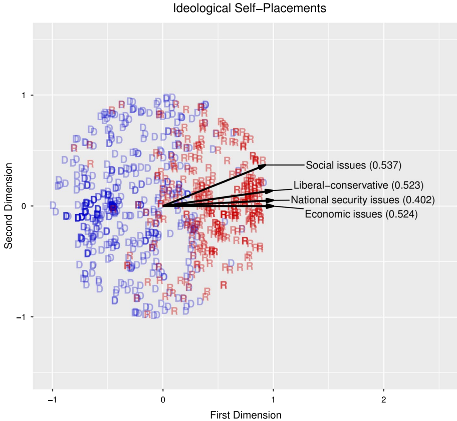
Fig. 5 Ordered Optimal Classification scaling of the 2015 Cooperative Congressional Election Study data. Democratic (D) and Republican (R) respondents shown alongside the selected ideological question normal vectors (with PRE fit statistics in parentheses)
