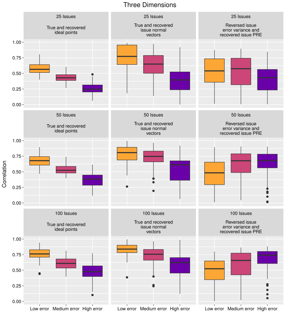
Fig. 9 Monte Carlo tests of Ordered Optimal Classification performance in three dimensions with 25, 50, and 100 issues
