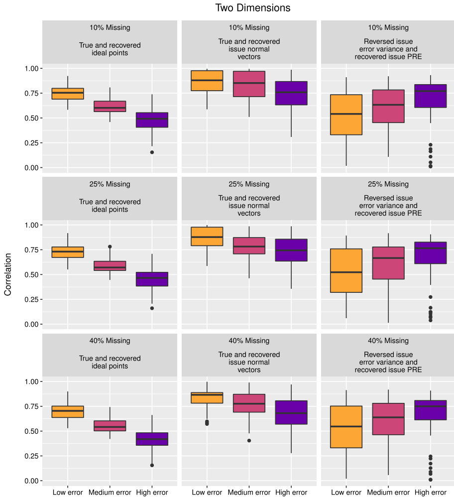
Fig. 3 Monte Carlo tests of Ordered Optimal Classification performance in two dimensions
