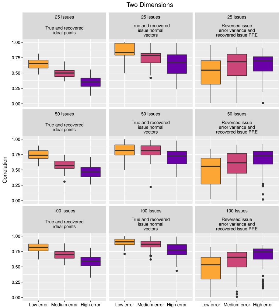
Fig. 8 Monte Carlo tests of Ordered Optimal Classification performance in two dimensions with 25, 50, and 100 issues
