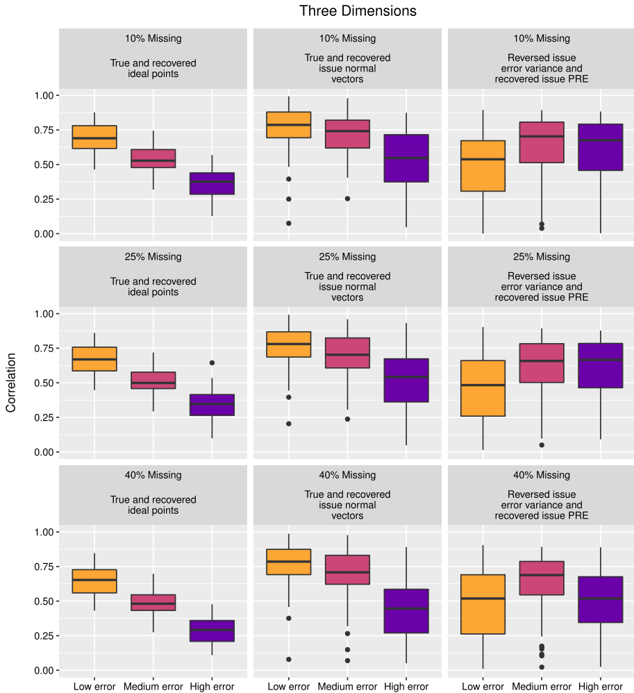
Fig. 4 Monte Carlo tests of Ordered Optimal Classification performance in three dimensions
