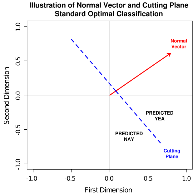
Fig. 1 Illustration of standard (binary) Optimal Classification. The cutting plane (the dashed blue line) defines the prediction surface, while the normal vector (the solid red line) is perpendicular by construction and indicates the direction or orientation of the issue in the latent ideological space. (Color figure online)
